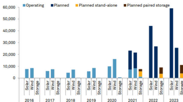
Figure 5: Annual installed capacity of wind, solar and battery storage, 2016-2023
